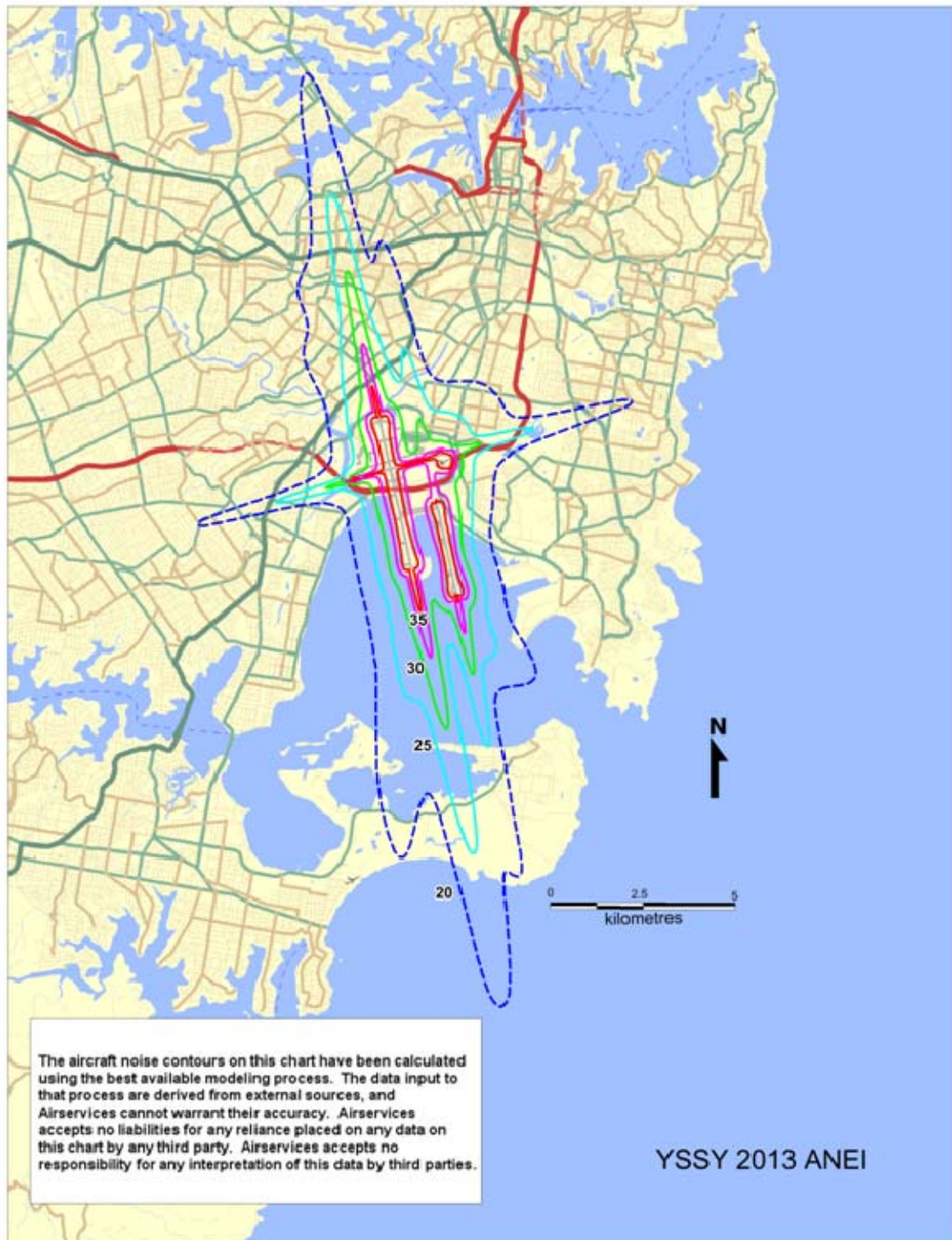
ANEI contours modelled by INM 7.0d incorporating terrain data.
