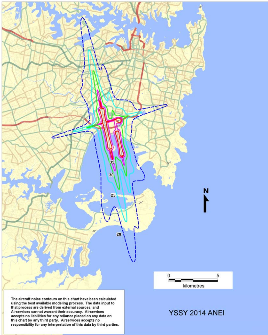
ANEI contours modelled by INM 7.0d incorporating terrain data.
